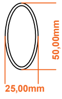
A SECTION
