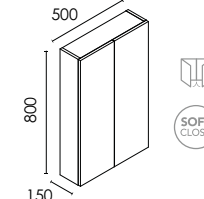
500MM DAI 2 DOOR WALL UNIT W500 x H800 x D150
