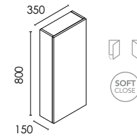
350MM DAI 1 DOOR WALL UNIT W350 x H800 x D150
