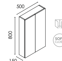
500MM DAI 2 DOOR WALL UNIT W500 x H800 x D150 ○ F10900 Gloss White £422 ● F11068 Matt Sand £422 ● F10902 Nordic Oak £422 ● F10901 Samara Ash £422
